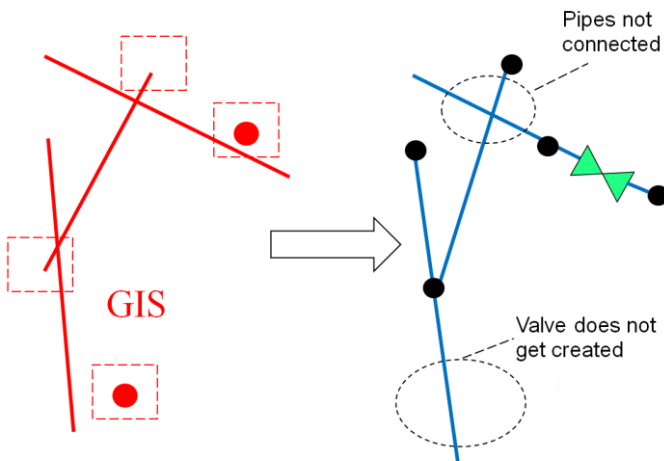
Figure 8 – Splitting
